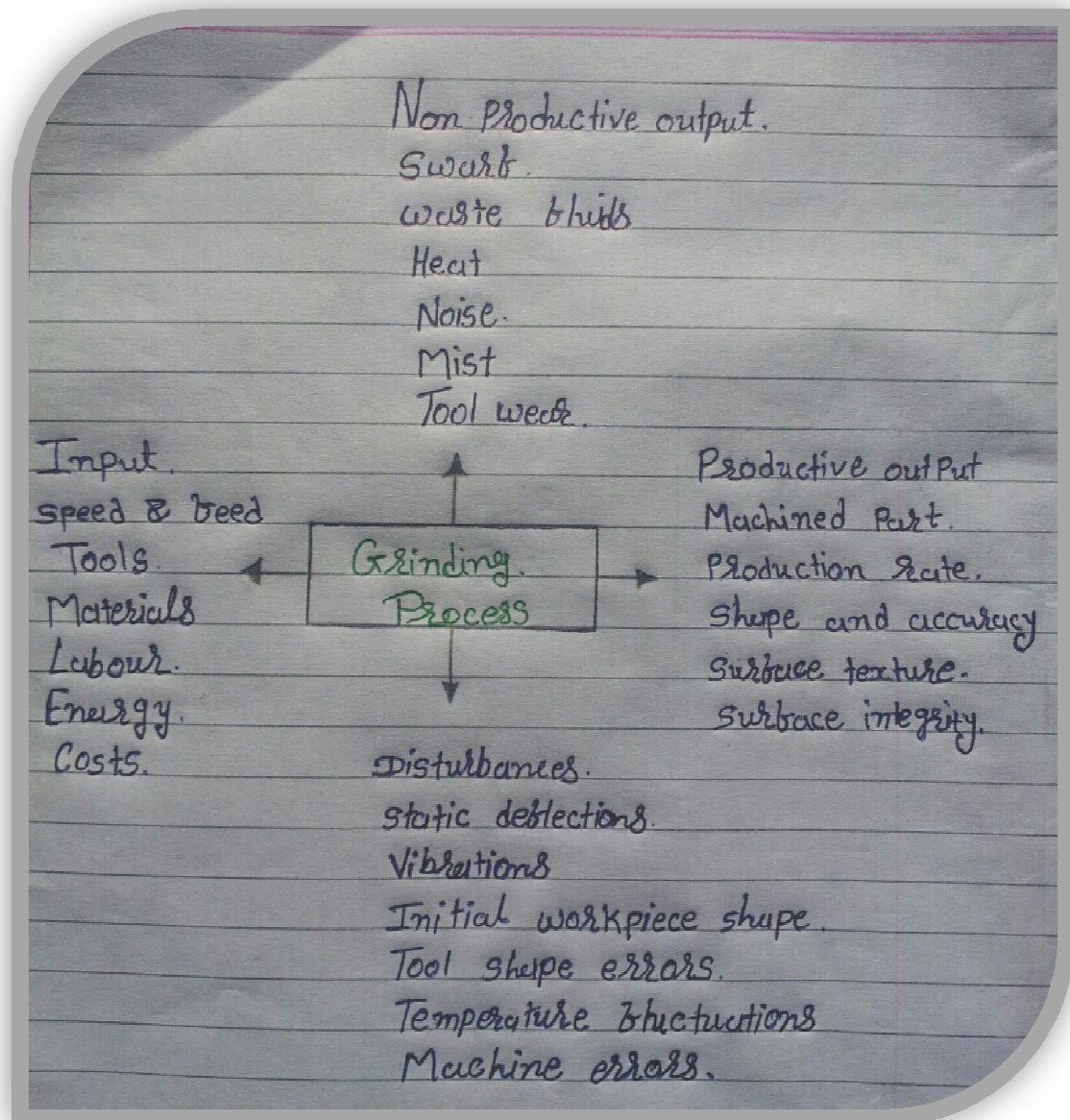
Figure 2. Inputs and Outputs of a Grinding Process
